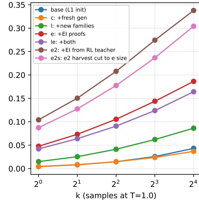
Dolci gate valid@k
