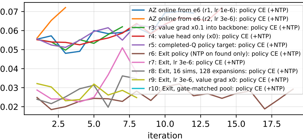
policy loss
