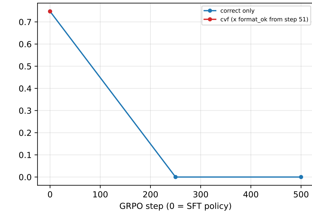
cvf — Dolci gate, training benches (700 items)
