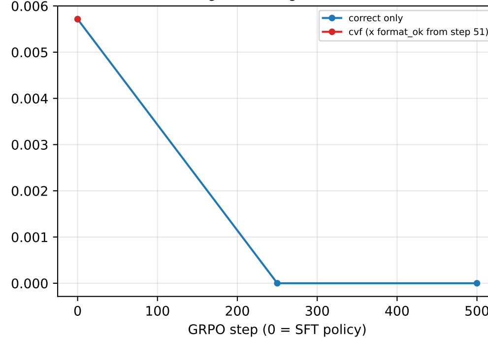
valid — Dolci gate, dapo + knowledge (250 items, OOD)
