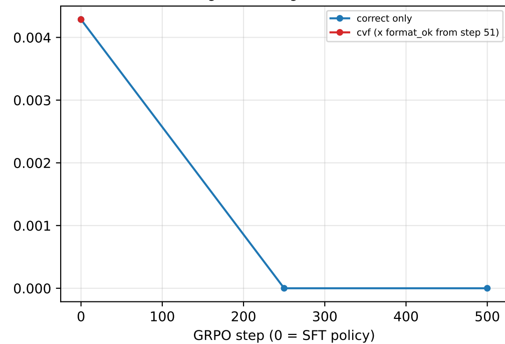
cvf — Dolci gate, dapo + knowledge (250 items, OOD)
