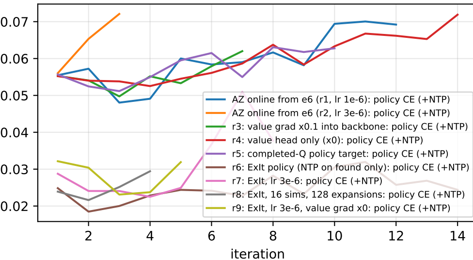
policy loss
