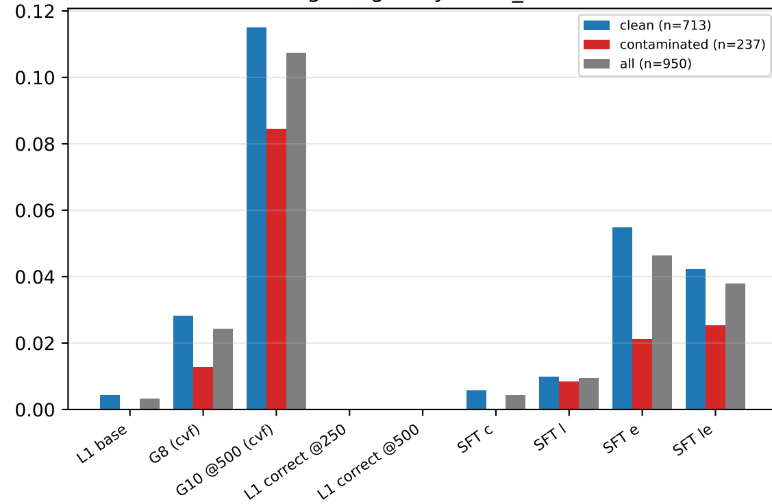
Dolci gate, greedy: valid_correct
