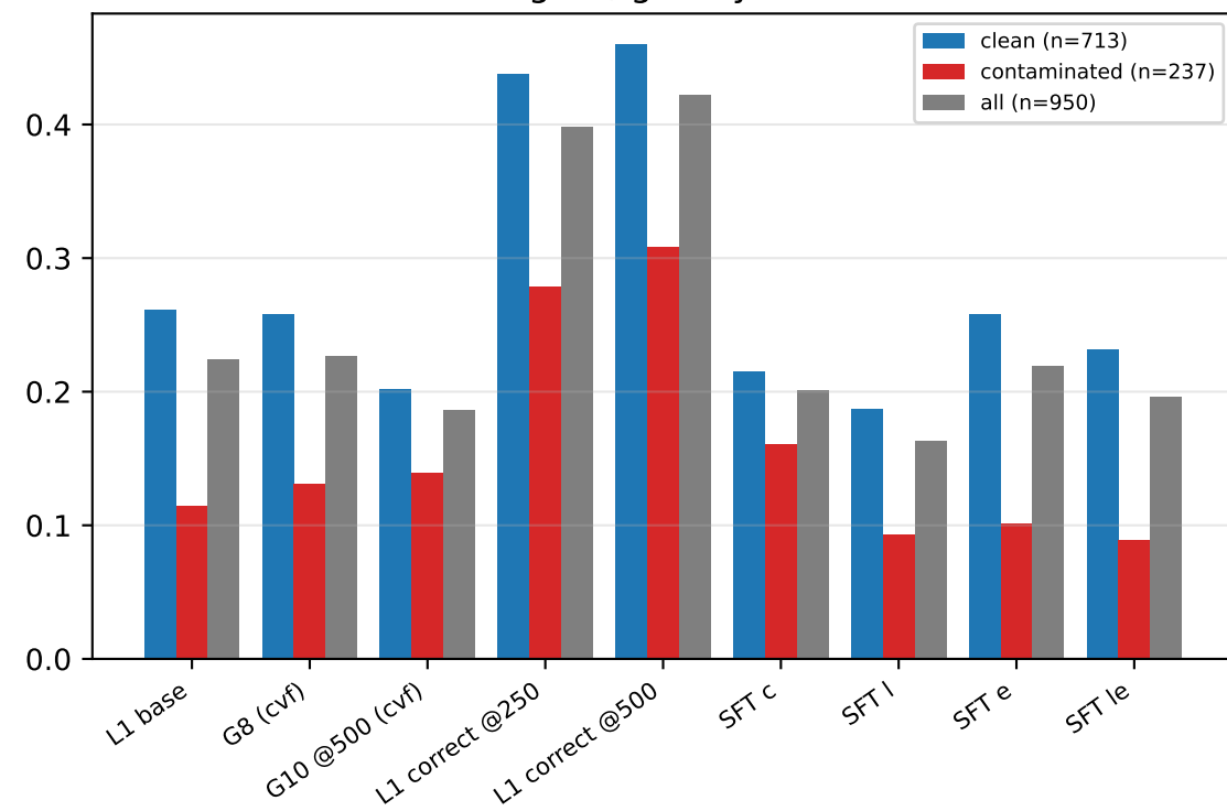
Dolci gate, greedy: correct
