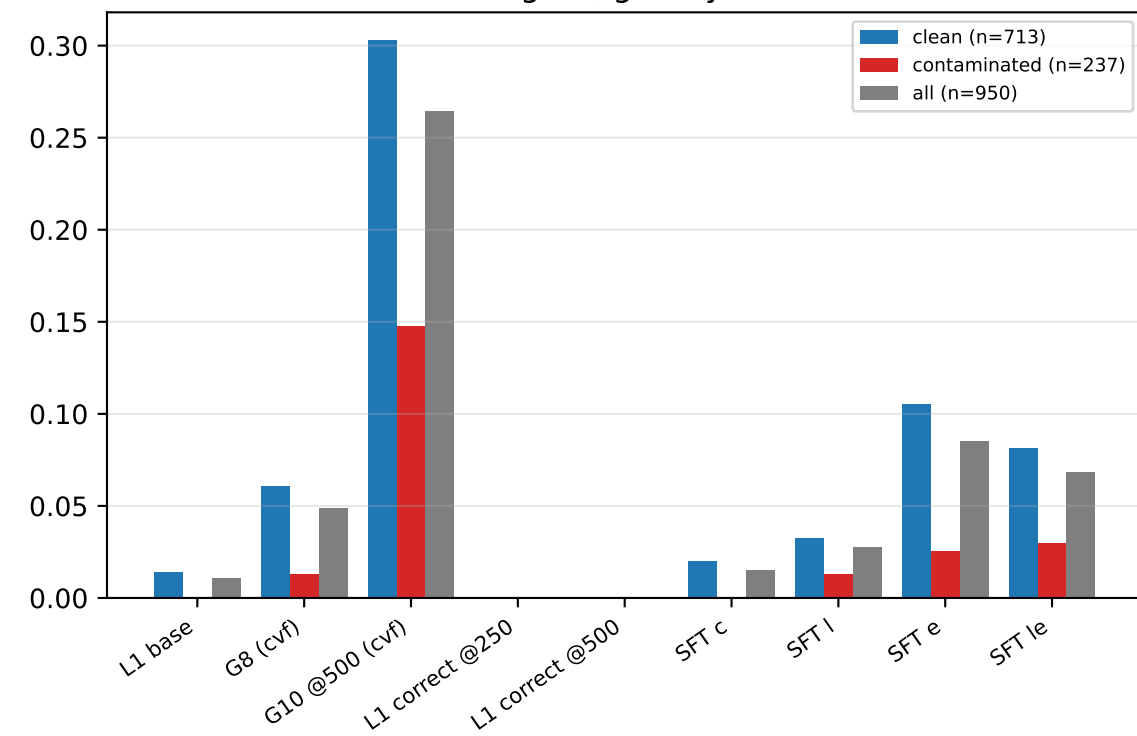
Dolci gate, greedy: valid
