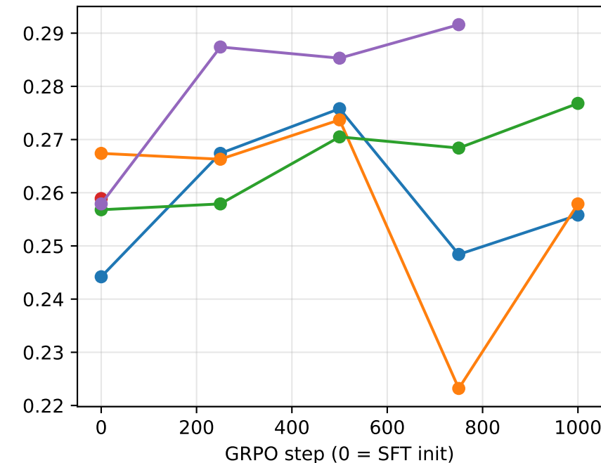
correct (clean, n=713)
