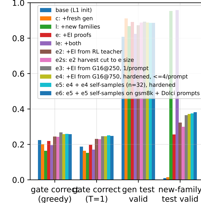
side effects: correctness and in-domain validity
