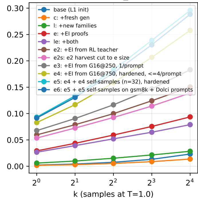
Dolci gate valid_correct@k
