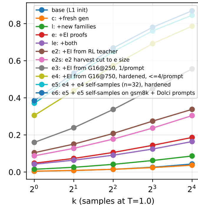
Dolci gate valid@k
