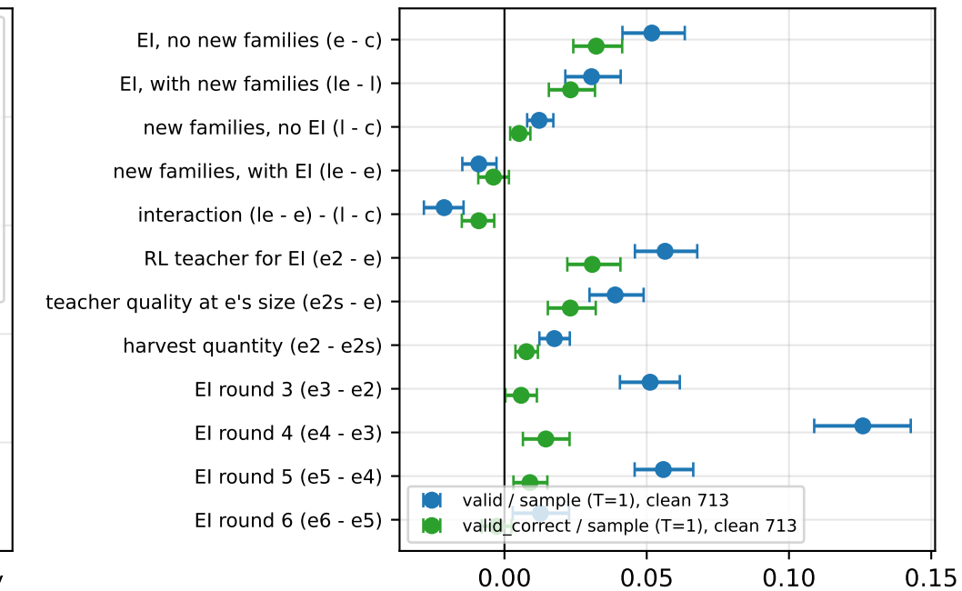
2x2 contrasts, 95% paired-bootstrap CI
