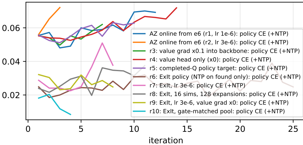
policy loss
