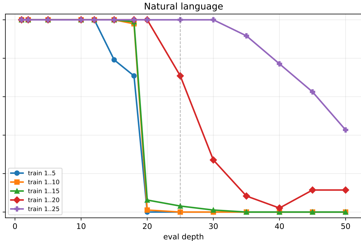
Joint valid+correct@16 by eval depth
