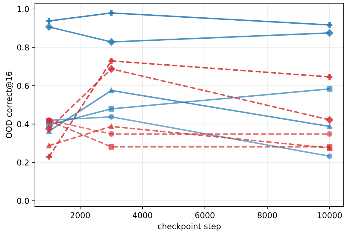
Seed 3407 intermediate checkpoint curves
