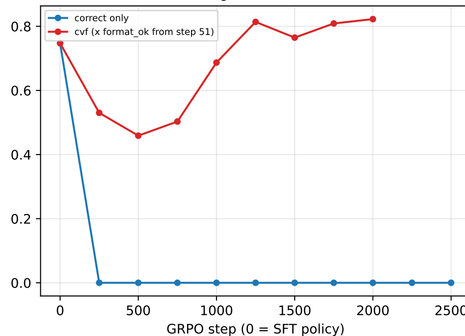
cvf — Dolci gate, training benches (700 items)
