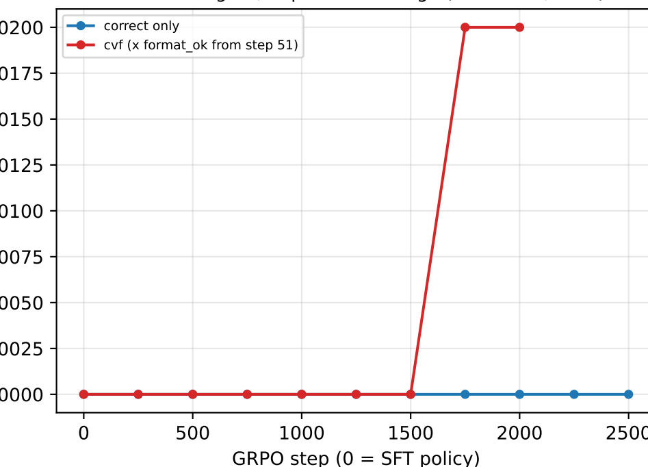
cvf — Dolci gate, dapo + knowledge (250 items, OOD)
