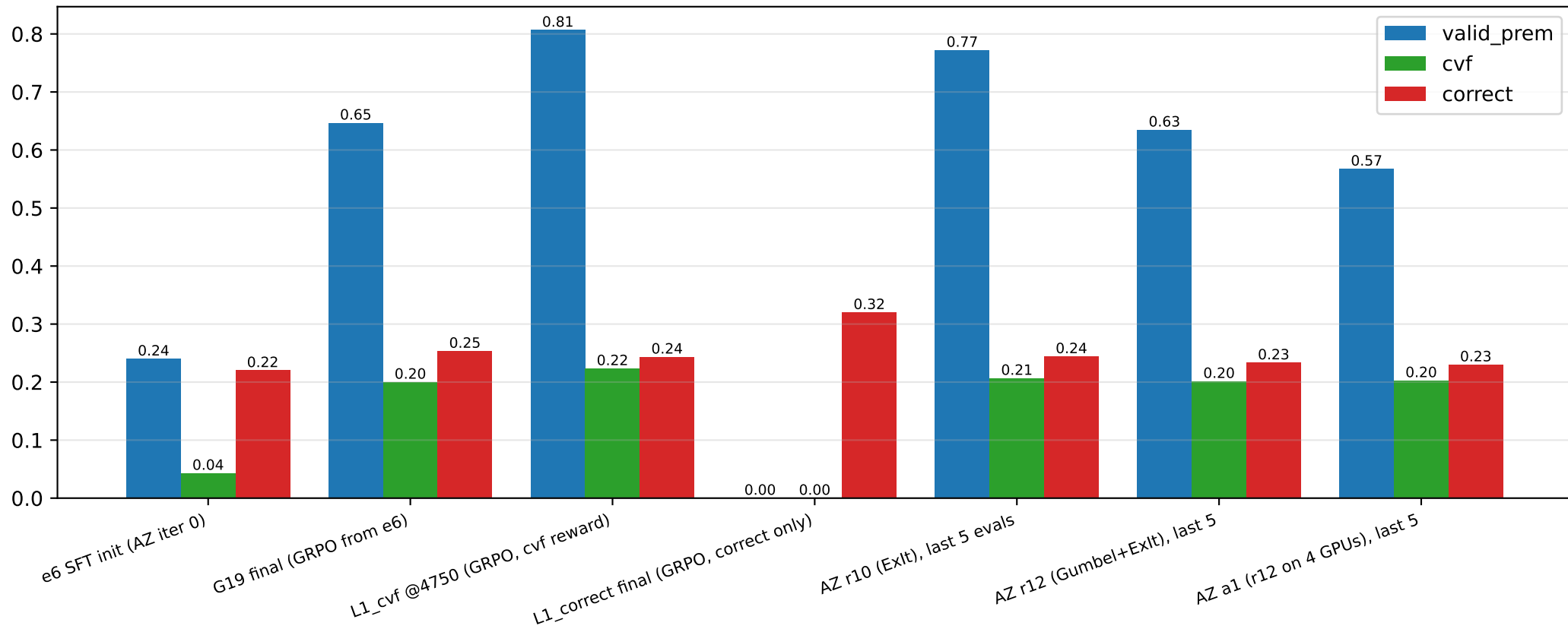
Same 300 held-out gate items, same scorer (libext checker): AZ = GRPO; correctness stuck at init
