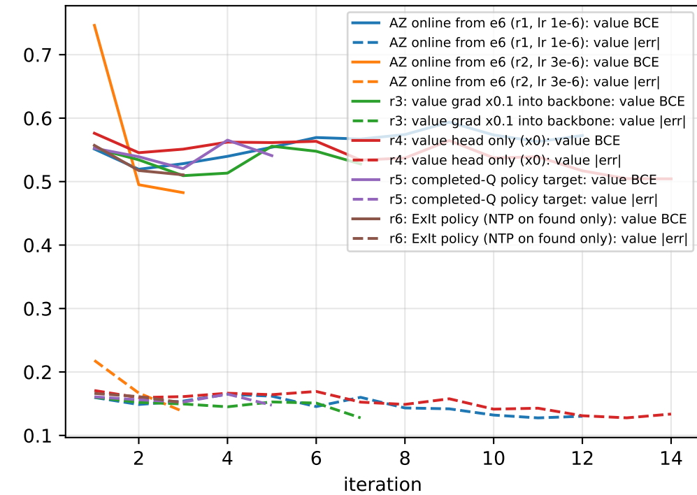
cost
