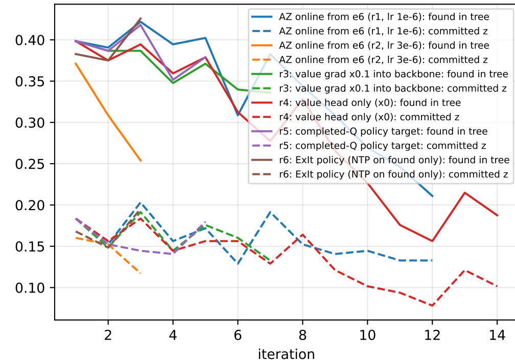
policy loss
