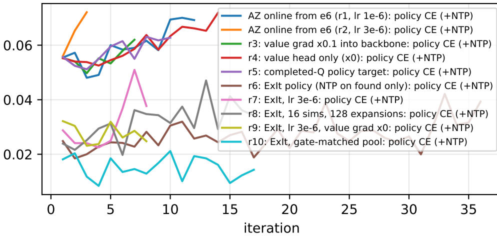
policy loss
