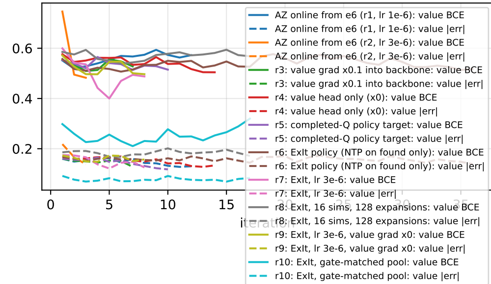
value loss
