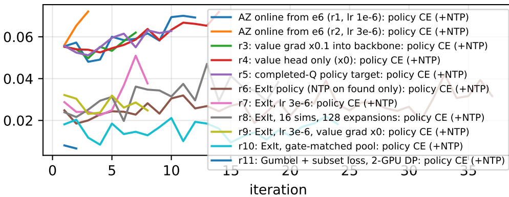
policy loss
