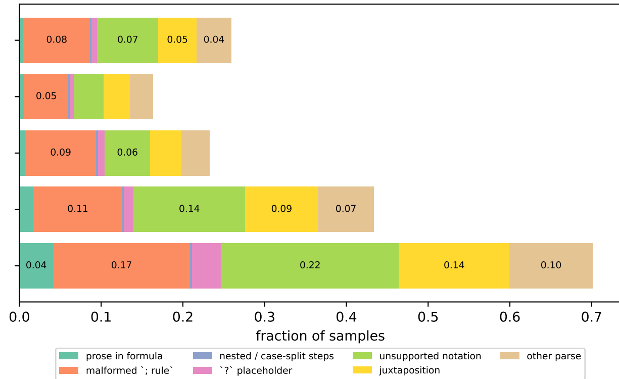
parse errors by kind (share of all samples)
