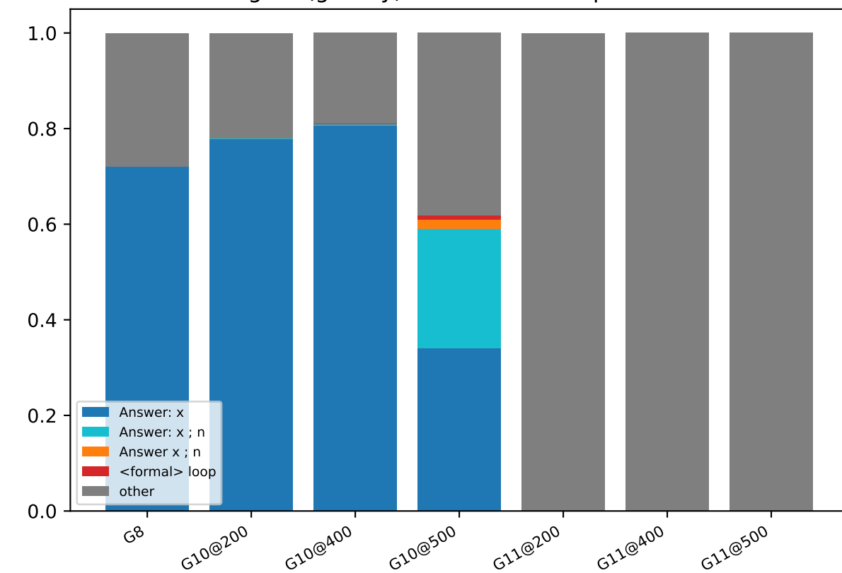
gate (greedy): what follows </proof>
