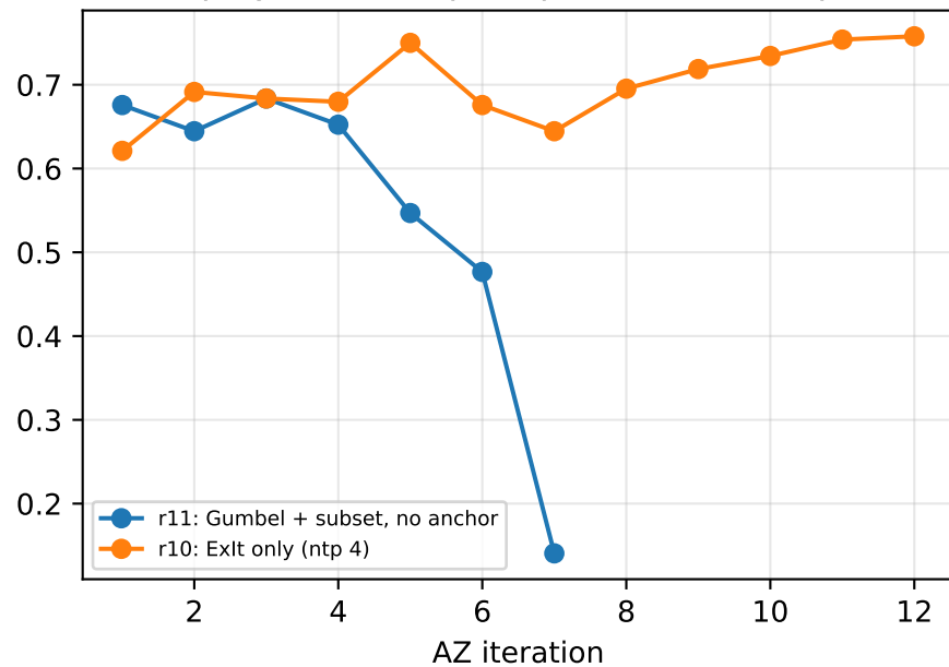
self-play: share of prompts with a valid proof
