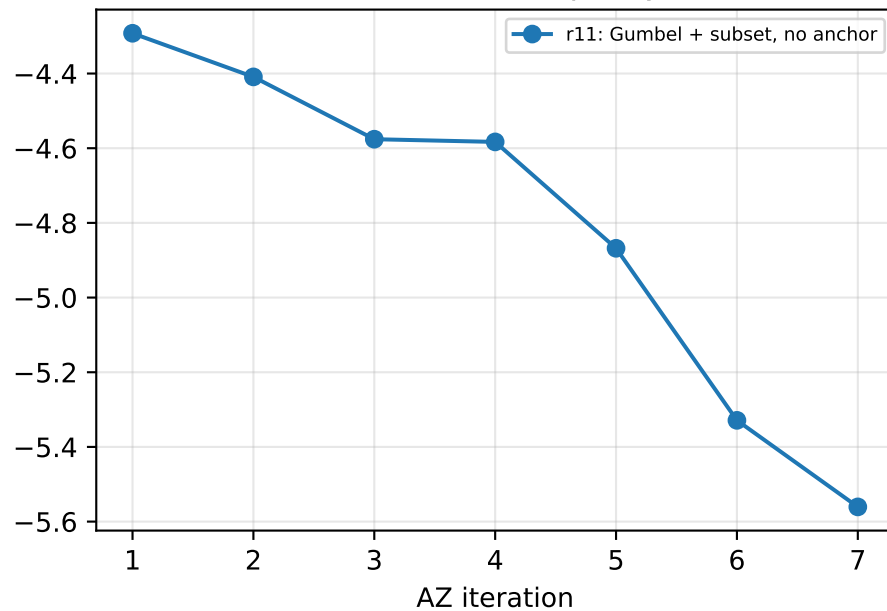
mean log-prob of sampled legal lines (lower = flatter policy)
