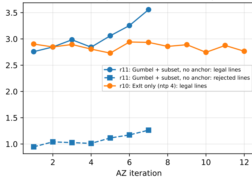
distinct lines per move (of K=8 samples)
