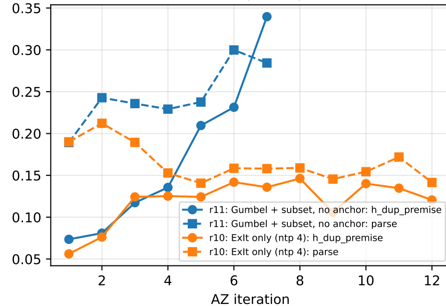
checker fails per expansion
