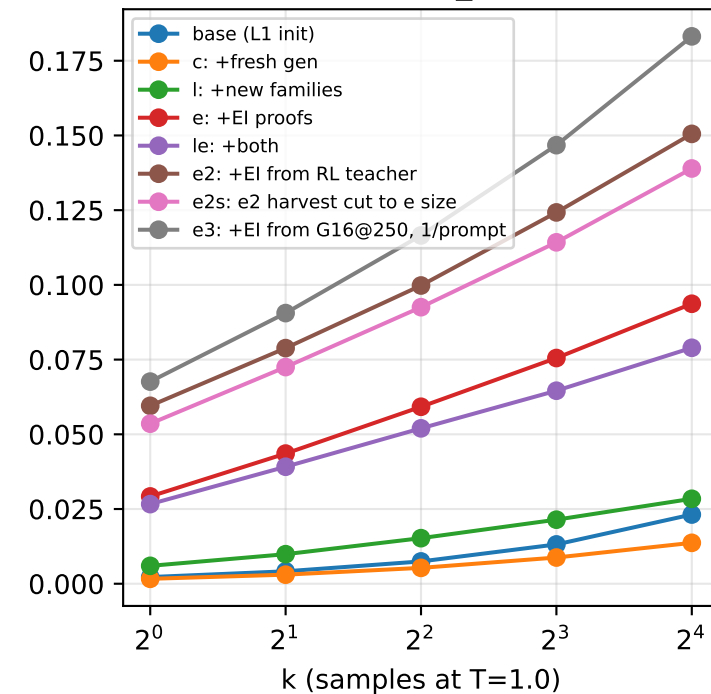
Dolci gate valid_correct@k
