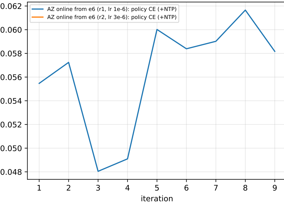
policy loss
