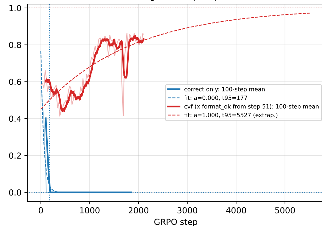
cvf — Dolci prompts (math, wordprob, yesno)
