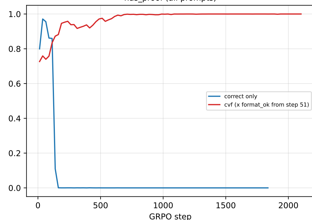
has_proof (all prompts)
