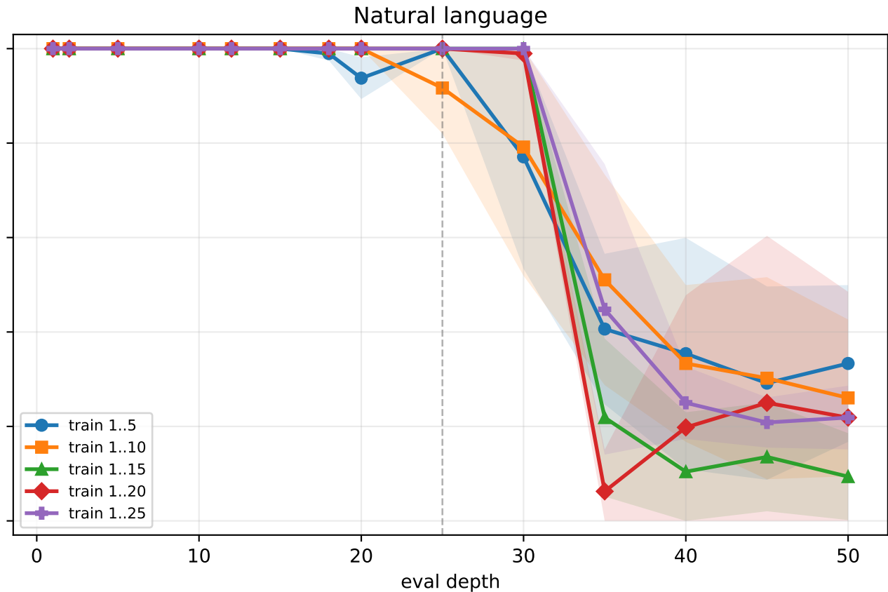
Correct@16 by eval depth
