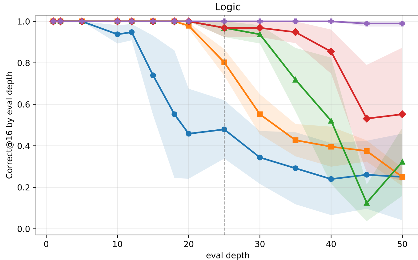
Correct@16 by eval depth
