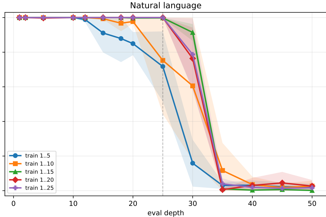
Sampled pass@1 correct and valid by eval depth
