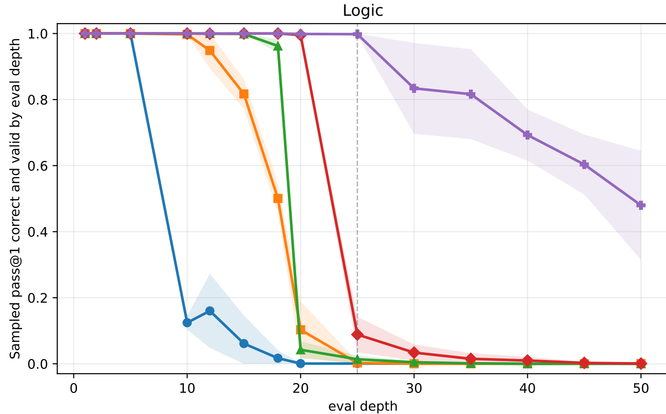
Sampled pass@1 correct and valid by eval depth
