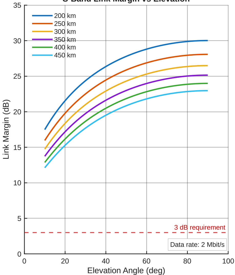
S-Band Link Margin vs Elevation
