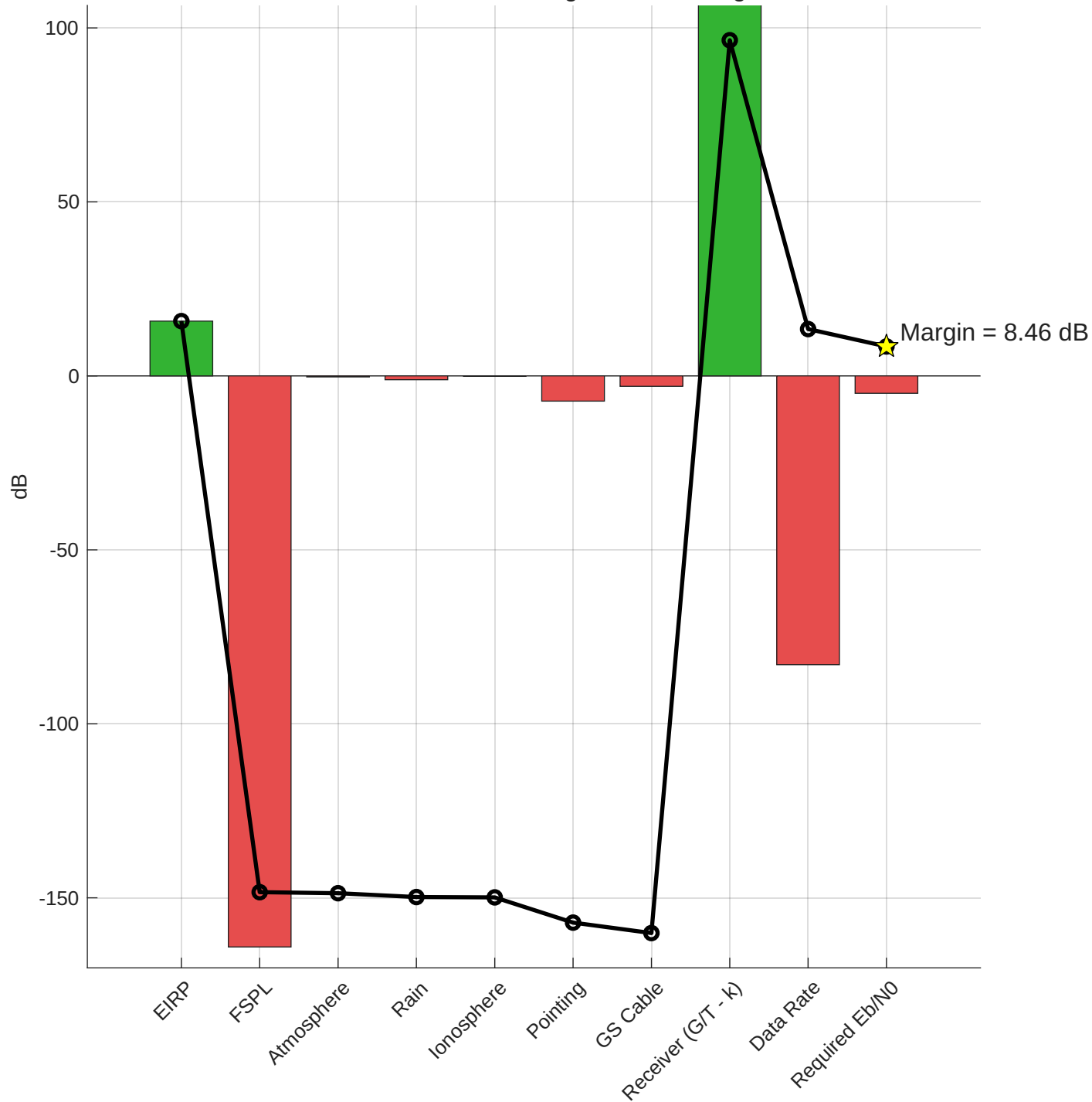
X-Band: Downlink Link Budget Waterfall Diagram
