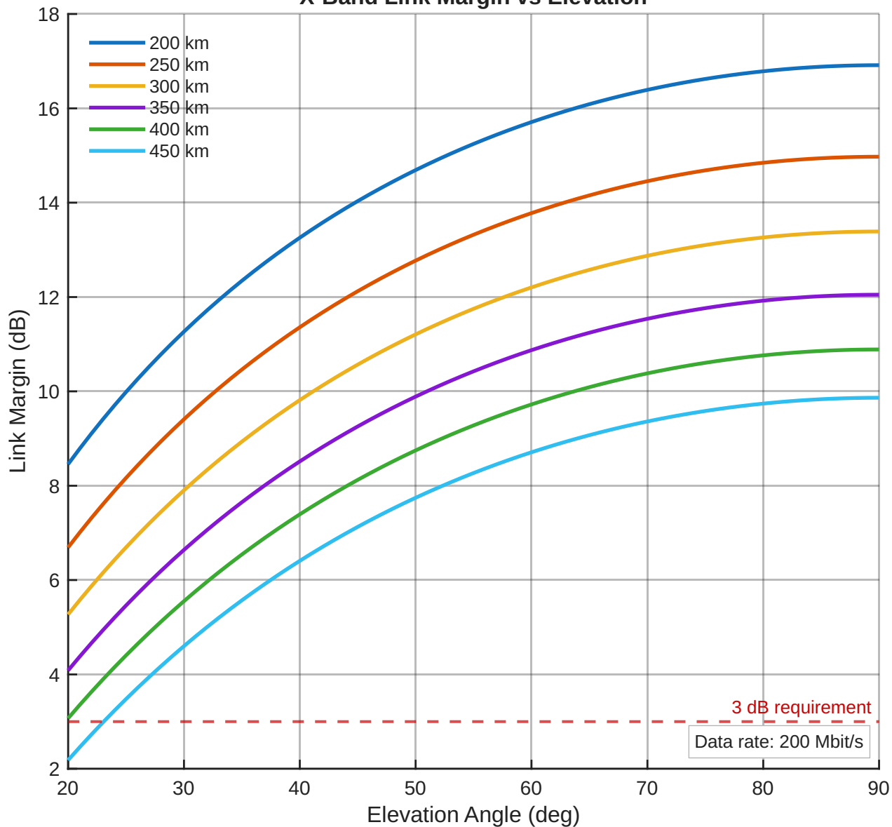
X-Band Link Margin vs Elevation
