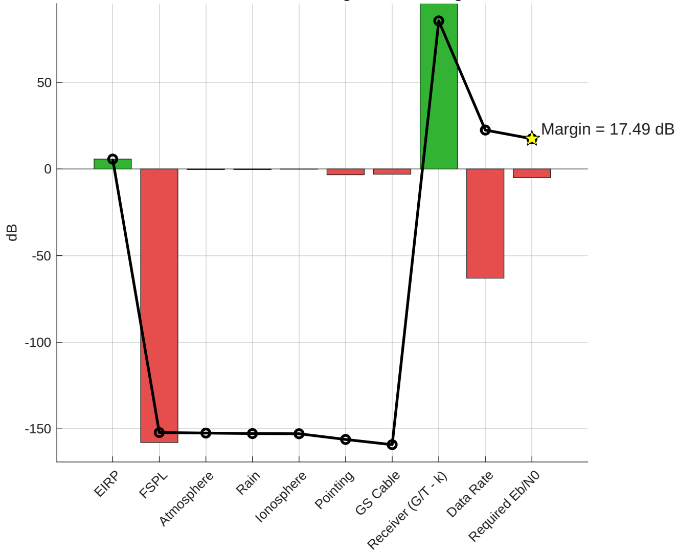
S-Band: Downlink Link Budget Waterfall Diagram
