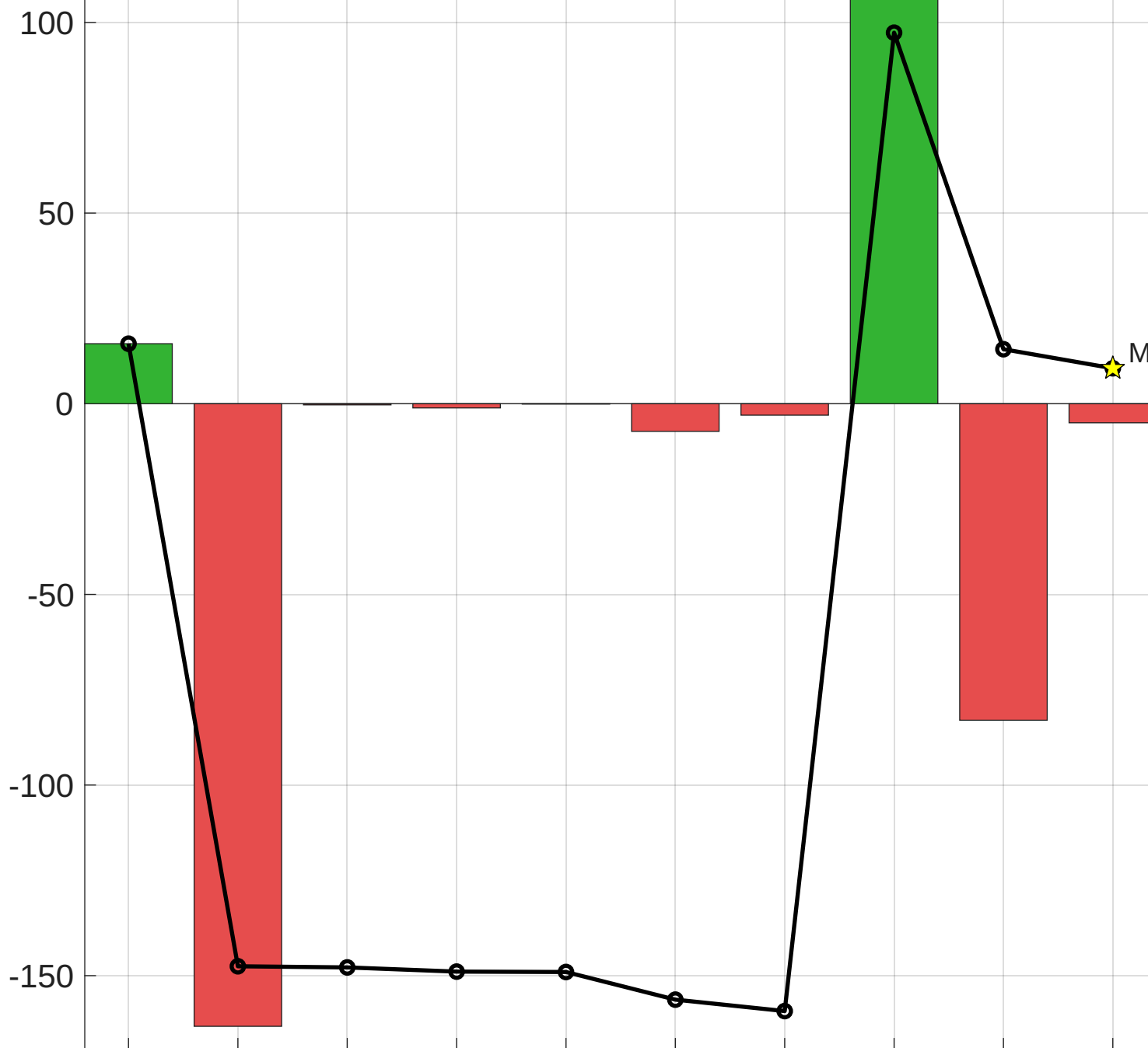
X-Band: Downlink Link Budget Waterfall Diagram
