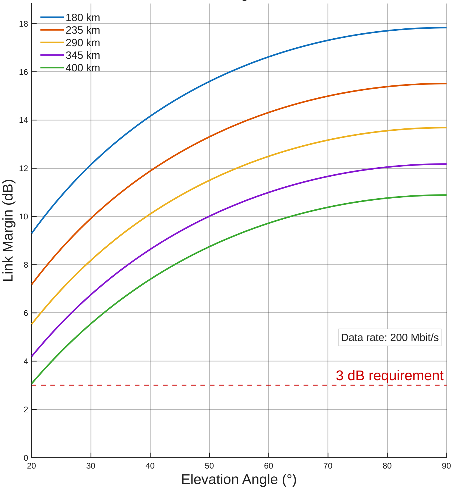
X-Band Link Margin vs Elevation
