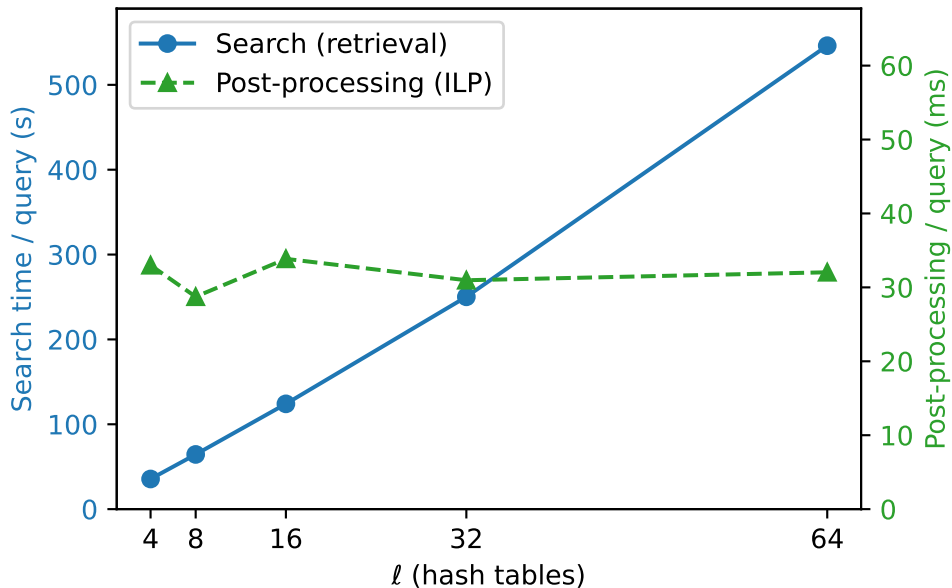
1B SIFT: query time vs \ell (100% feasible)
