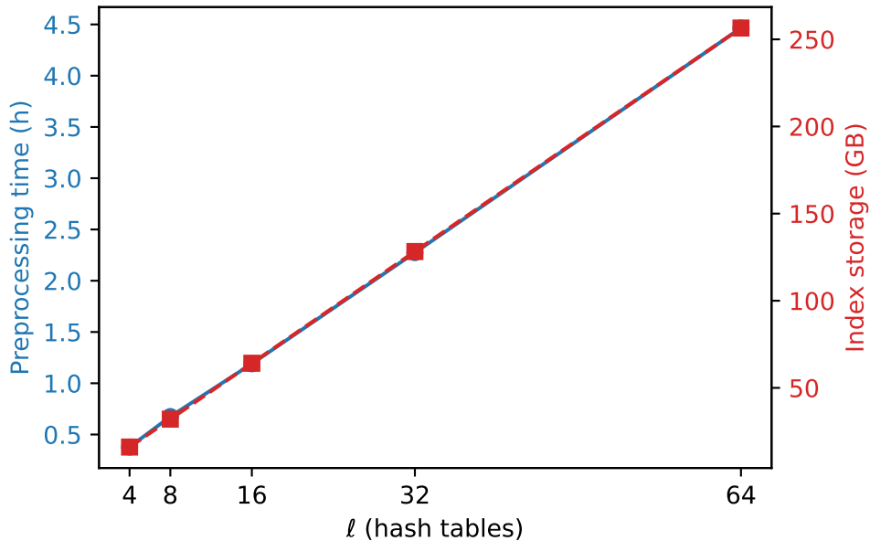
Synthetic 1B (d=32): preprocessing & storage
