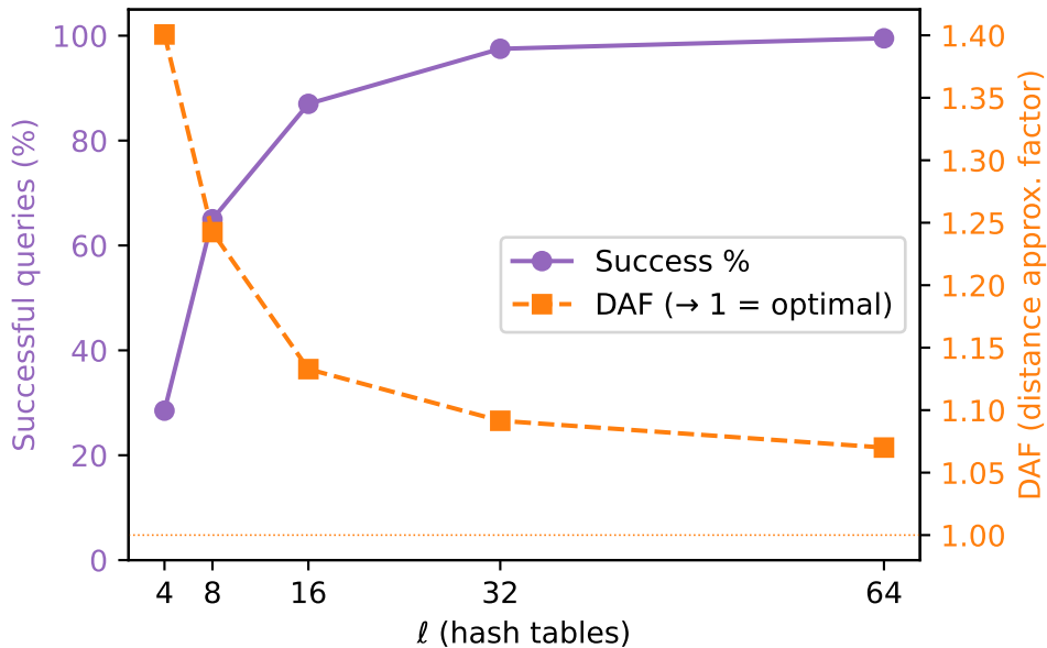
Synthetic 1B (d=32): feasibility & quality vs \ell
