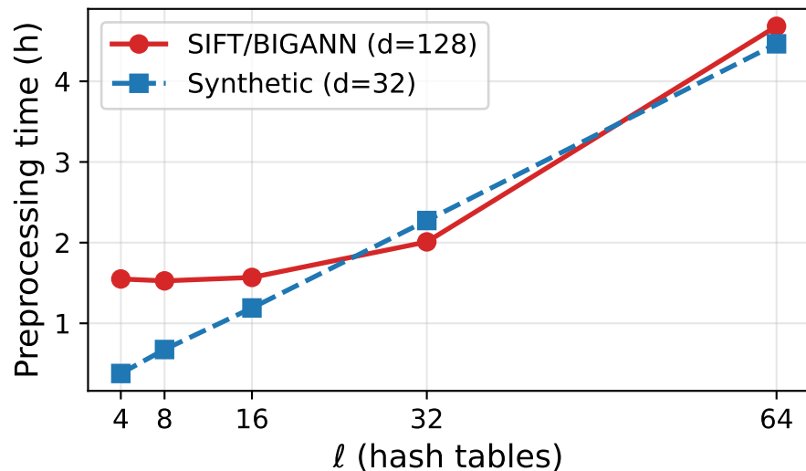
(a) Build time vs \ell
