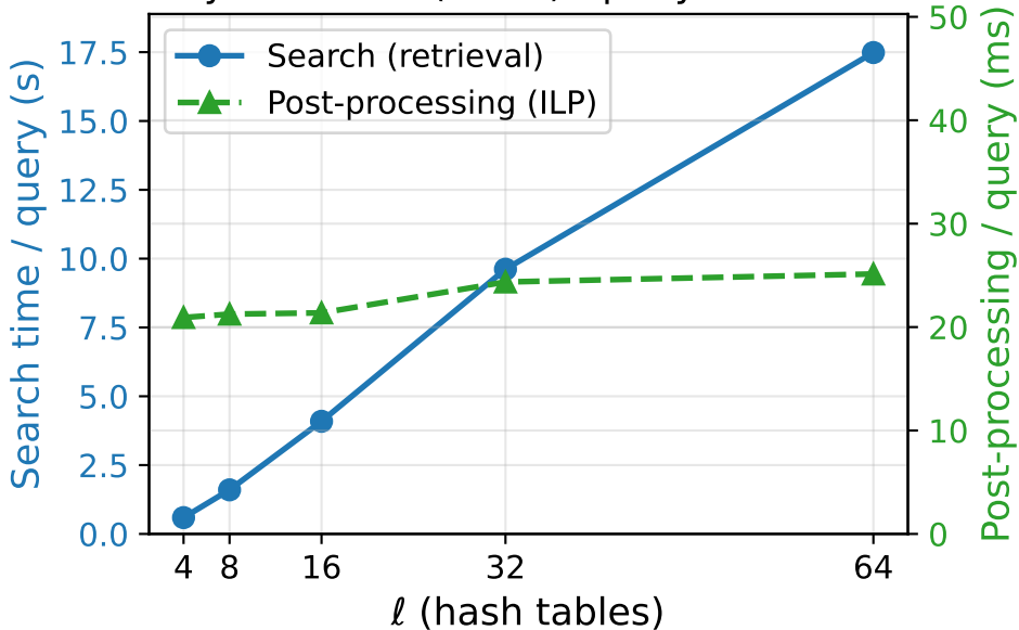
Synthetic 1B (d=32): query time vs \ell
