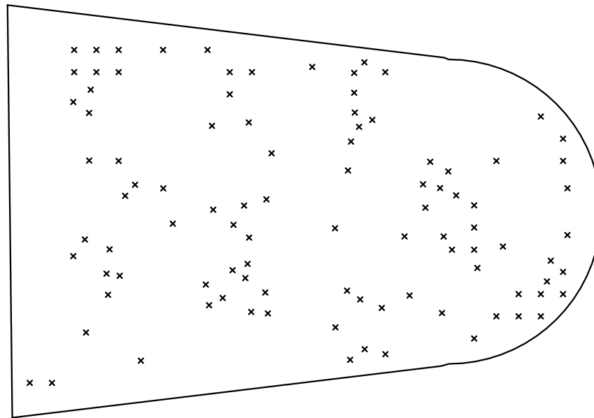
Drill Map: x 0.300mm / 0.0118" (97 holes)
