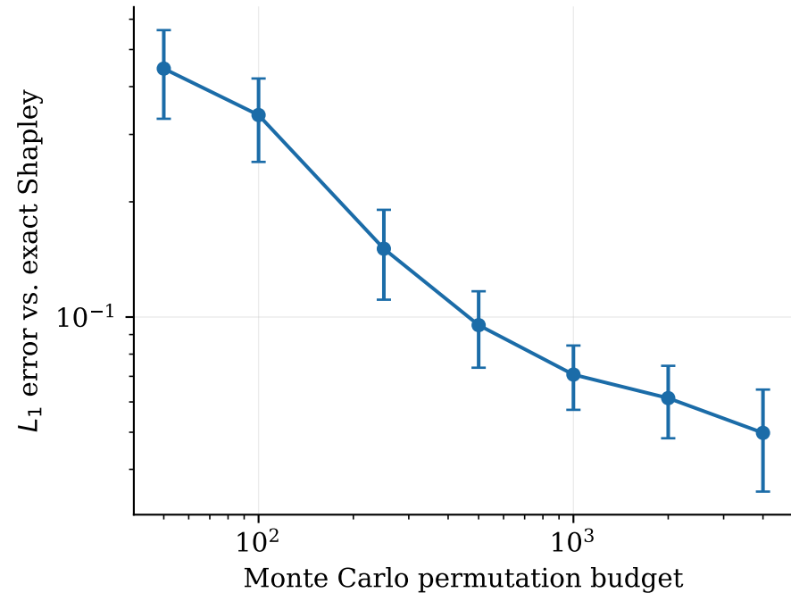
(a) Convergence ( n=10 firms, 8 seeds/point)
