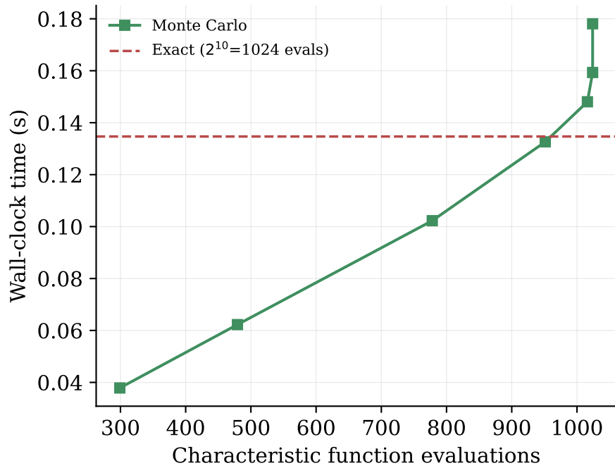
(b) Computational cost
