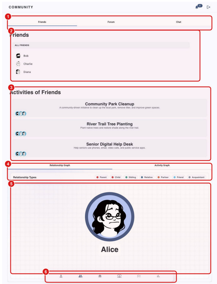
Figure 4. Community screen showing friendships, shared activities and relationship analysis.
