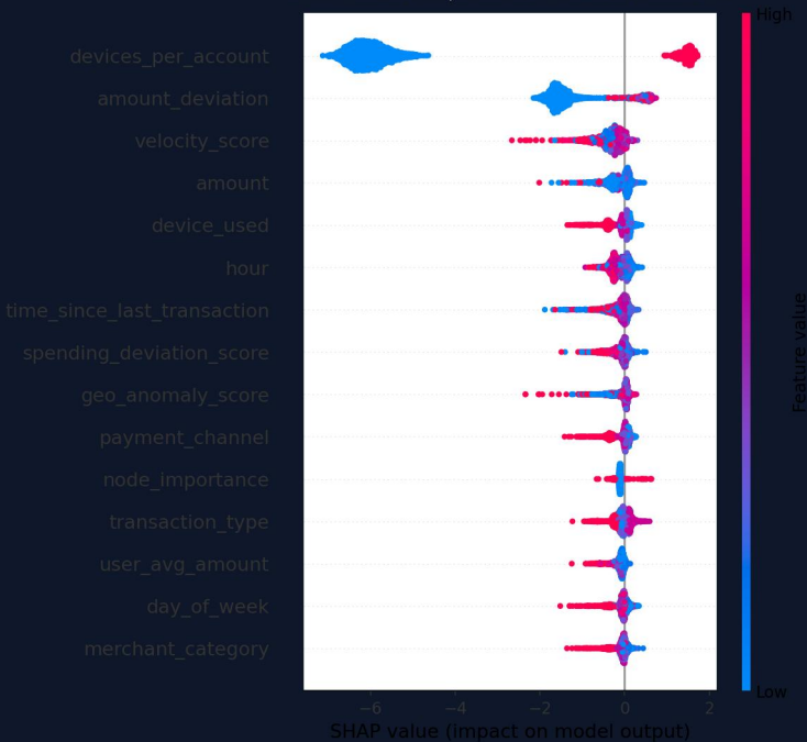
SHAP Feature Importance - XGBoost (GuardAI)
