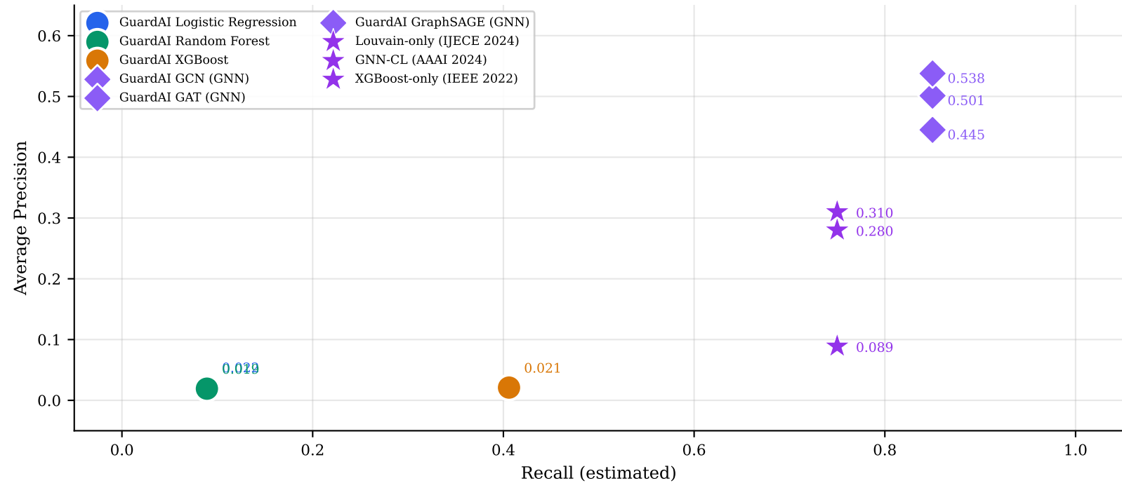
Fig. 4: Precision-Recall Comparison vs. Published Benchmarks
