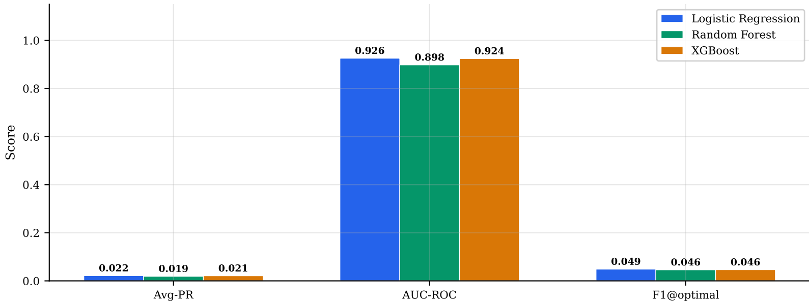
Fig. 1: Model Performance Comparison (PaySim, 150k rows)
