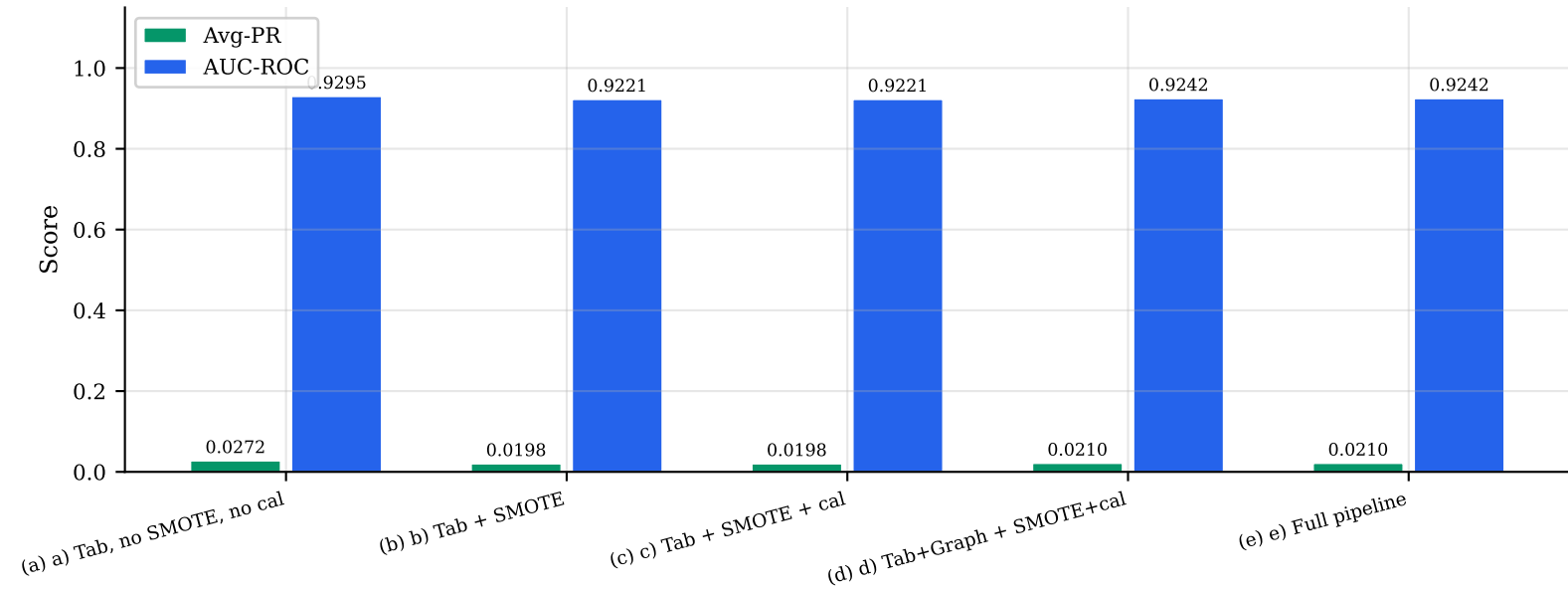
Fig. 3: 5-Step Ablation Study (XGBoost)
