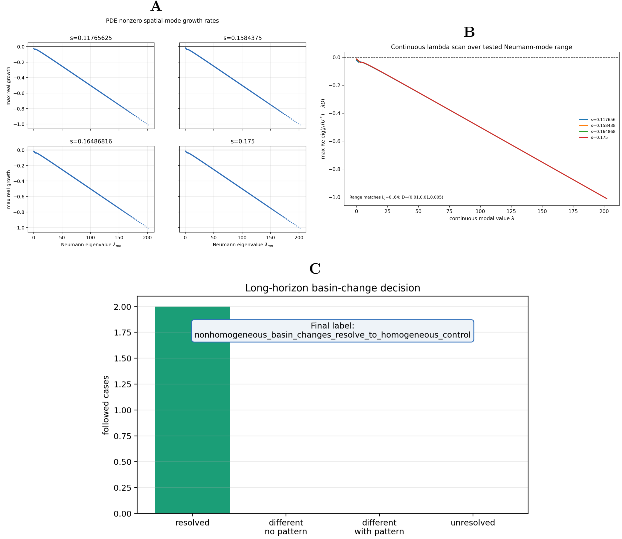
Figure 4: Spatial-mode and finite-amplitude PDE tests. Panel A plots maximum real growth rates for tested discrete Neumann modes, computed from J_F(U^*) - \lambda_{ij}D . Panel B shows the continuous \lambda -scan over 600 equally spaced values in the mode-equivalent range corresponding to i, j = 0, \dots, 64 . Panels A and B support tested-range linear spatial stability for the current diffusion coefficients. Panel C summarizes long-horizon follow-up of the two finite-amplitude heterogeneous cases that changed finite-horizon basin labels; both resolved to their matched homogeneous controls without persistent spatial patterning. These diagnostics do not exhaust all possible modes, diffusion coefficients, or heterogeneous initial conditions.
