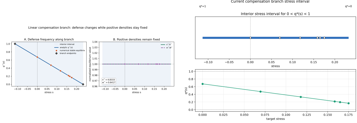
Figure 1: Compensation branch and stress interval. The left subfigure plots q^*(s) against numerical stable persistent equilibria and shows normalized n^* and w^* , which remain effectively fixed along the linear branch. The right subfigure plots the stress interval where 0 < q^*(s) < 1 . These panels support branch feasibility and analytic/numerical agreement in the tested parameterization; they do not imply global stability or feasibility for all trade-offs.
