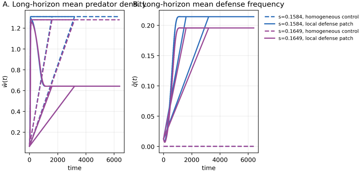
Figure 11: Long-horizon mean time series for the finite-horizon basin-changing non-homogeneous cases. The followed cases are the targeted cases selected from the earlier finite-amplitude tests, not a broad PDE scan.
