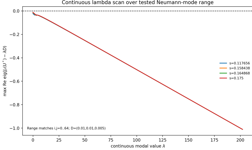
Figure 6: Continuous \lambda -scan for J_F(U^*) - \lambda D over 600 equally spaced \lambda values in the mode-equivalent range corresponding to i, j = 0, \dots, 64 . This scan strengthens the tested spatial-mode result over that range, but it is still a tested-range diagnostic rather than a proof for all possible modes or diffusion coefficients.
