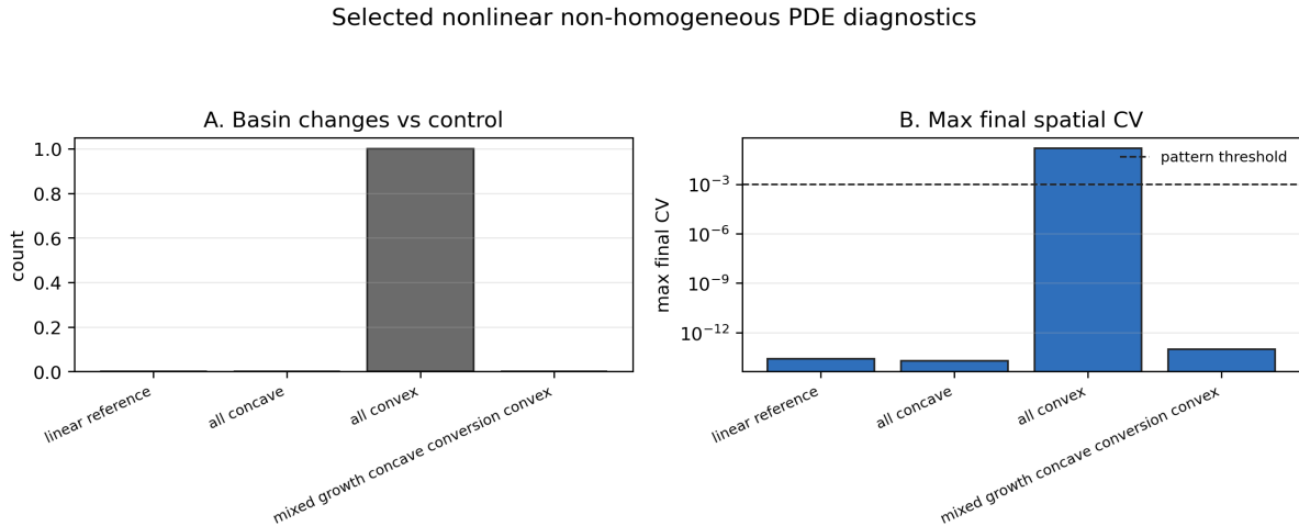
Figure 17: Selected nonlinear non-homogeneous PDE diagnostics. This supporting figure reports targeted finite-amplitude checks for selected nonlinear branches and does not establish global robustness to heterogeneous initial conditions.
