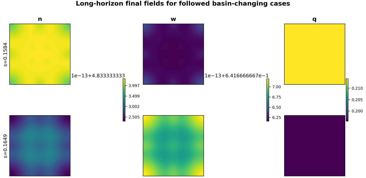
Figure 13: Long-horizon final fields for the followed basin-changing cases. These diagnostics support resolution without persistent spatial patterning for the followed cases.
