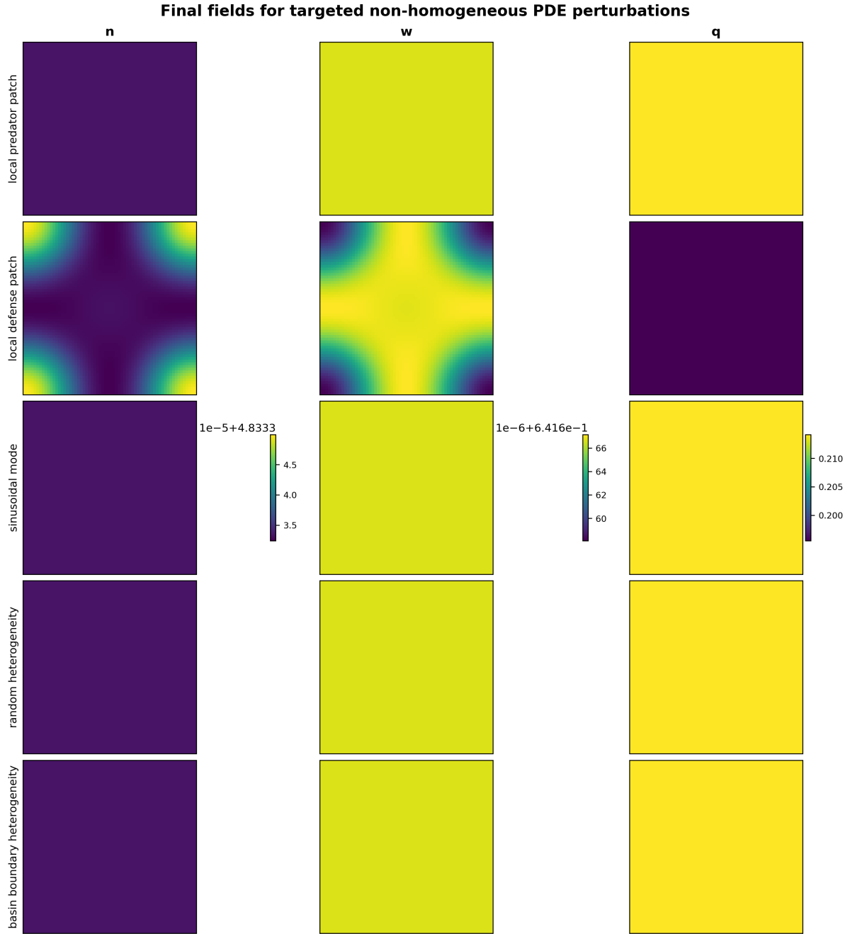
Figure 8: Final PDE fields for representative targeted non-homogeneous perturbation tests. This diagnostic figure supports the absence of persistent spatial patterning in the displayed cases, but it is not a proof for all heterogeneous initial conditions.
