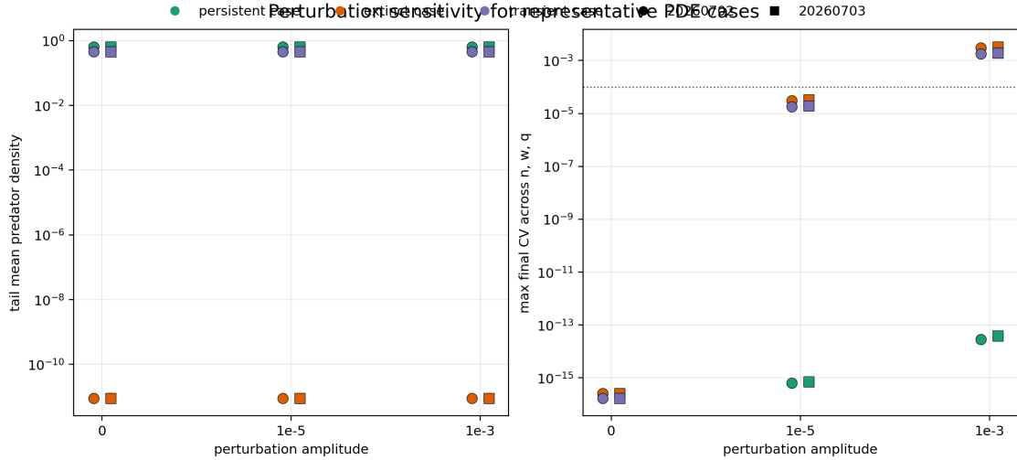
Figure 4: Perturbation-amplitude and seed sensitivity for the representative PDE cases.
