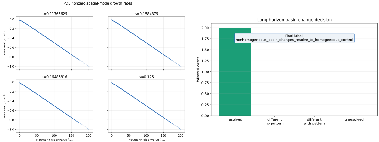
Figure 4: Spatial-mode and finite-amplitude PDE tests. The left panel plots maximum real growth rates for tested Neumann modes, computed from J_F(U^*) - \lambda_{ij}D . The right panel summarizes long-horizon follow-up of finite-amplitude heterogeneous basin-changing cases. These diagnostics support linear spatial stability and show that followed finite-horizon basin changes resolved without persistent spatial patterning; they do not exhaust all possible heterogeneous initial conditions.
