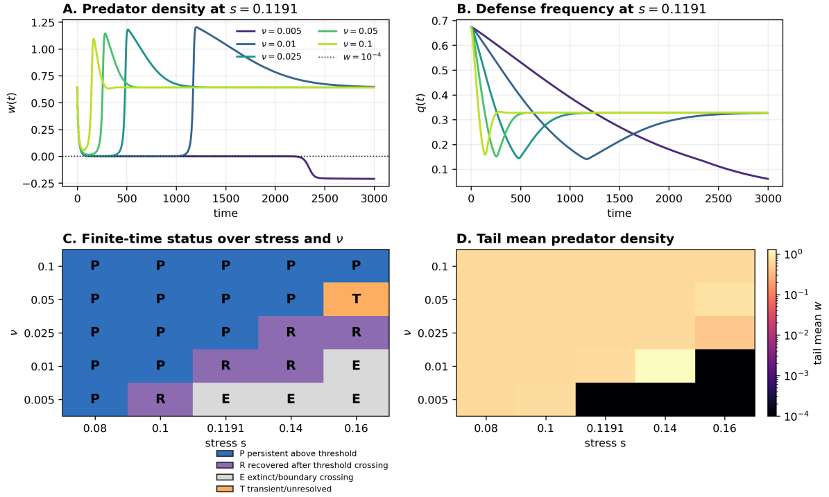
Figure 18: Finite-time evolutionary-rate sensitivity diagnostic. Panels A and B show w(t) and q(t) at s = 0.1191 ; the dotted line marks the extinction threshold. Panel C reports ecological finite-time status: P, persistent without threshold crossing; R, tail-persistent recovery after threshold crossing; E, extinct or boundary crossing; T, transient or unresolved. Panel D shows tail mean predator density across the small stress- \nu grid.
