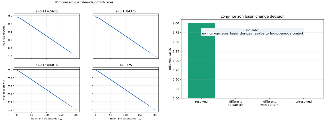
Figure 3: Spatial-mode and finite-amplitude PDE tests. The left panel plots maximum real growth rates for tested Neumann modes, computed from J_F(U^*) - \lambda_{ij}D . The right panel summarizes long-horizon follow-up of finite-amplitude heterogeneous basin-changing cases. These diagnostics support linear spatial stability and show that followed finite-horizon basin changes resolved without persistent spatial patterning; they do not exhaust all possible heterogeneous initial conditions.
