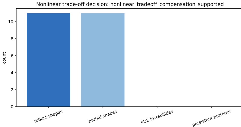
Figure 4: Controlled nonlinear trade-off extension summary. The figure summarizes branch recovery, shape-grid outcomes, and targeted PDE checks for selected nonlinear trade-off shapes. It supports compensation in selected nonlinear shapes while showing that the result remains local and parameter-sensitive; it does not prove the mechanism for all nonlinear trade-off functions.
