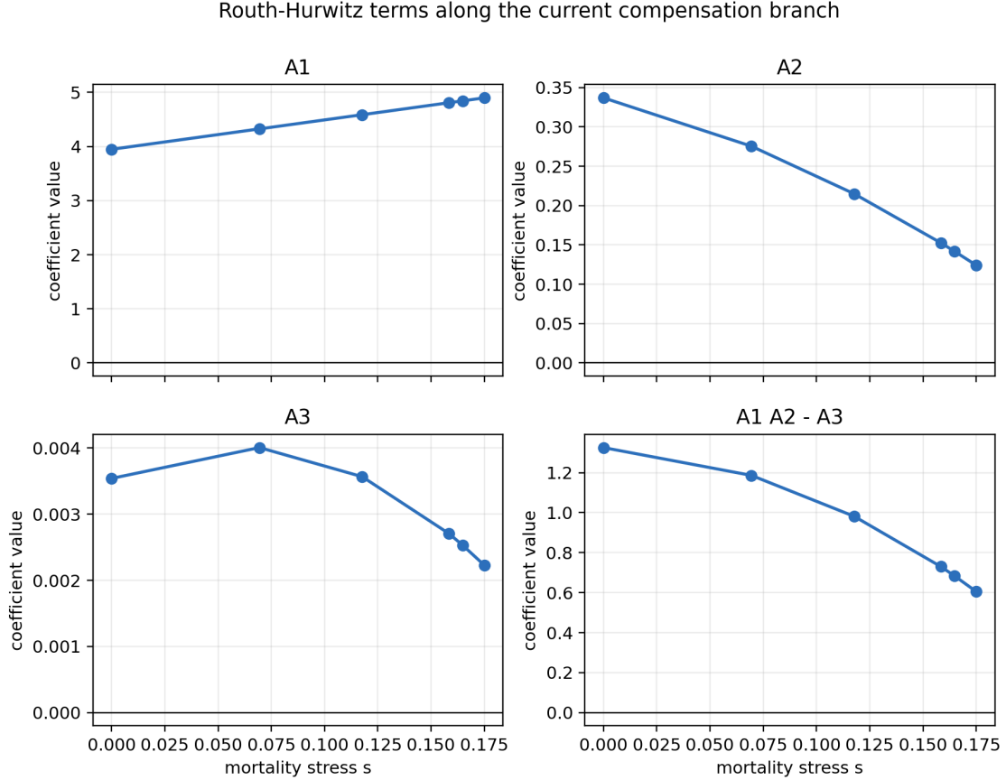
Figure 2: Routh–Hurwitz coefficient terms along the compensation branch. The plotted quantities are A_1 , A_2 , A_3 , and A_1 A_2 - A_3 . Their positivity supports local stability at the tested stresses; it does not establish global basin attraction or rule out other attractors.
