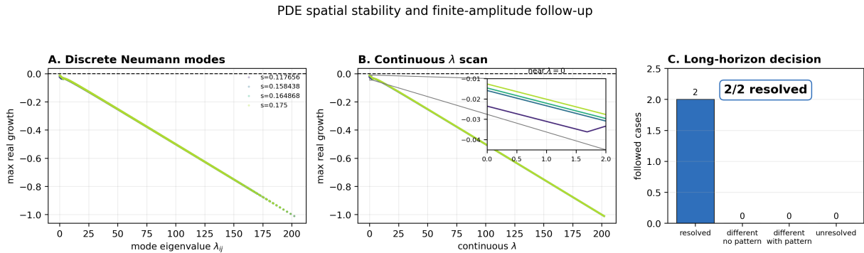
Figure 4: Spatial-mode and finite-amplitude PDE tests. Panel A plots maximum real growth rates for tested discrete Neumann modes, computed from J_F(U^*) - \lambda_{ij}D . Panel B shows the continuous \lambda -scan over 600 equally spaced values in the mode-equivalent range corresponding to i, j = 0, \dots, 64 . Panels A and B support tested-range linear spatial stability for the current diffusion coefficients. Panel C summarizes long-horizon follow-up of the two finite-amplitude heterogeneous cases that changed finite-horizon basin labels; both resolved to their matched homogeneous controls without persistent spatial patterning. These diagnostics do not exhaust all possible modes, diffusion coefficients, or heterogeneous initial conditions.
