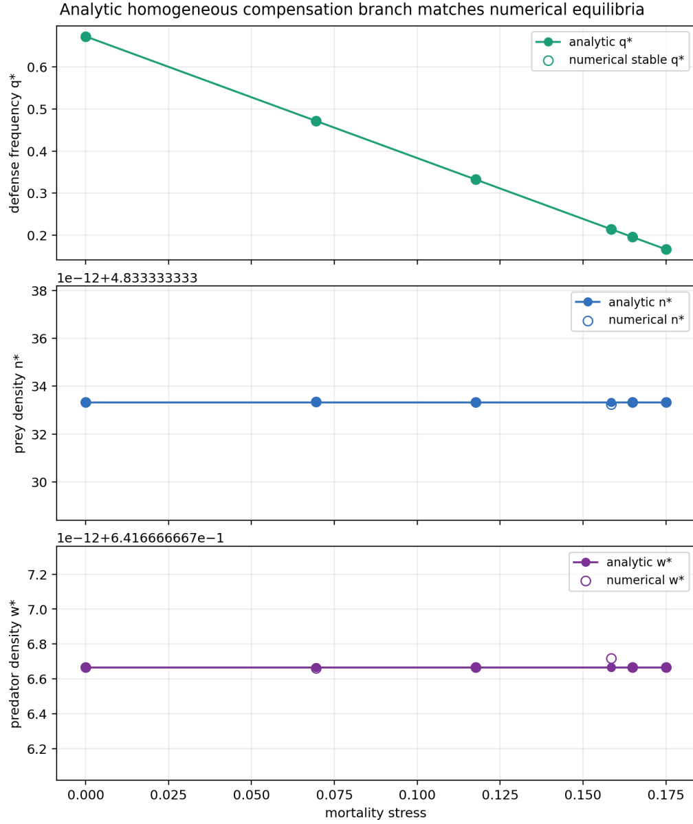
Figure 7: Analytic homogeneous compensation branch compared with the existing numerical stable persistent equilibria. The branch keeps n^* and w^* nearly fixed while q^*(s) declines with stress.
